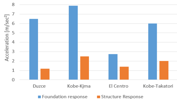
Figure IV-1 Reduction of peak acceleration response of foundation and superstructure in X-direction
