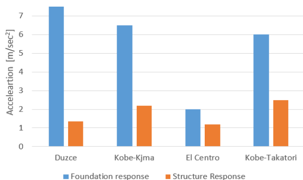
Figure IV-2 Reduction of peak acceleration response of foundation and superstructure in Y-direction
