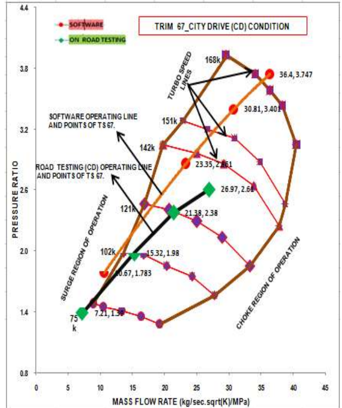
Fig. 4 Turbo-matching by simulation and at City Route
