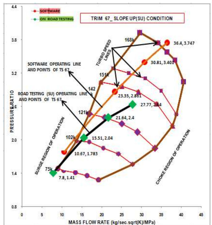
Fig. 5 Turbo-matching by simulation and at slope-up Route
