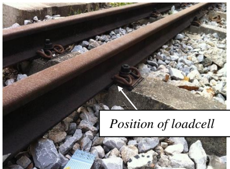
Fig. 3 Sensor installation location
