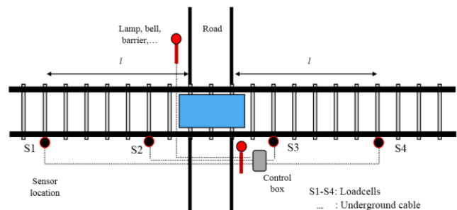
Fig. 1 The train alarm systems at the railway intersection
