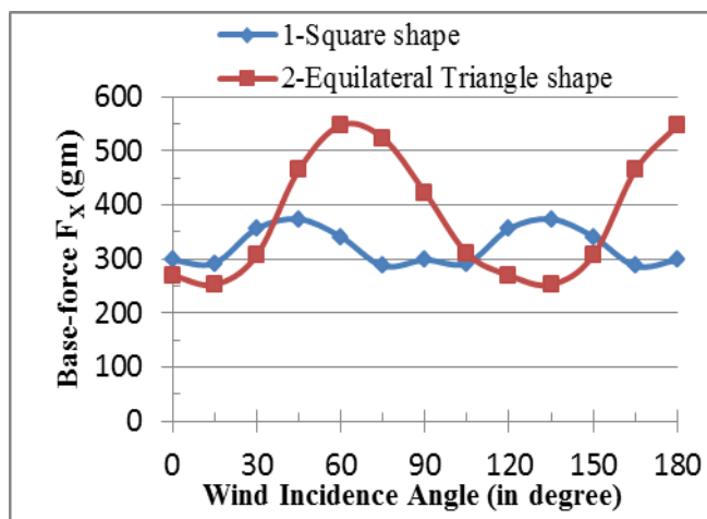
Fig. 4. Variation of along-wind force with wind incidence angle.
