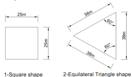
Fig. 1. Cross-sectional dimensions of prototype buildings with equal area.
