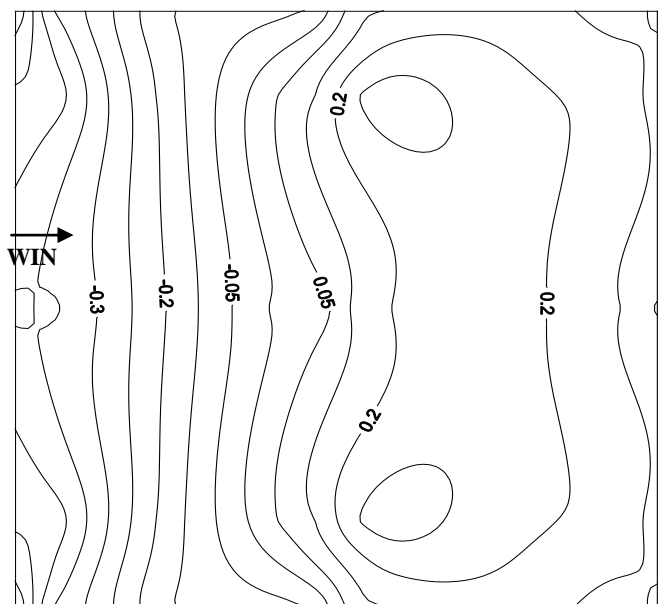
Fig.6 Contours of C_p on upper surface at 0° wind angle.
