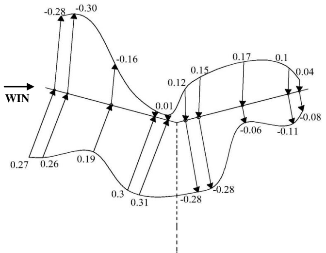
Fig.5 Cross sectional variation of C_p at mid section on upper and lower surface at 0° wind angle.
