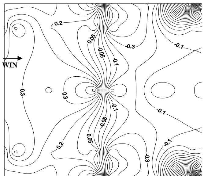
Fig.7 Contours of C_p on lower surface at 0° wind angle.
