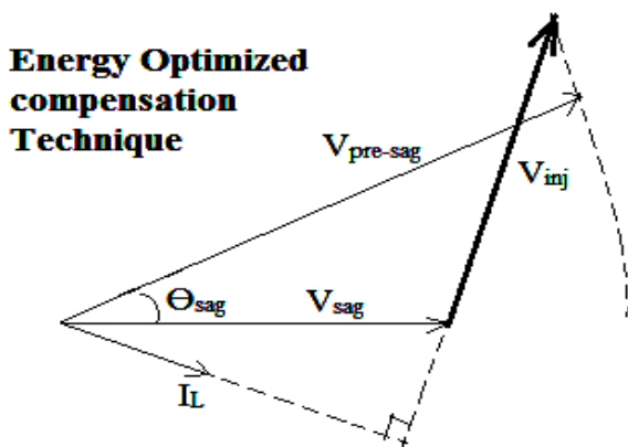
Figure.3: Conventional Control Strategies if DVR [9]
