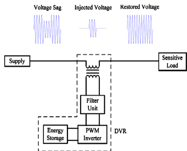
Figure.2: Typical application of DVR in distribution system
