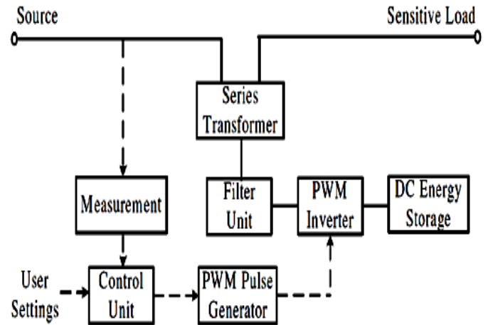
Figure.4: Simplified DVR block
