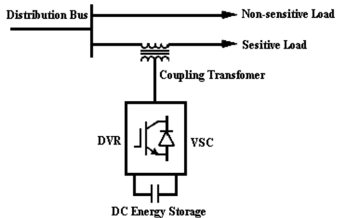
Figure.1: Basic Configuration of DVR
